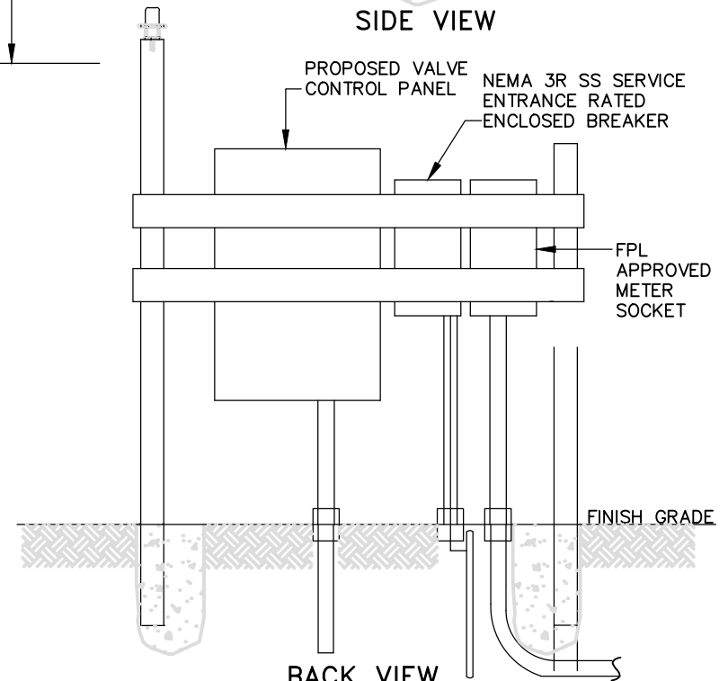
BACK VIEW
