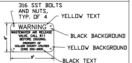
2 WARNING SIGN DETAIL NOT TO SCALE
