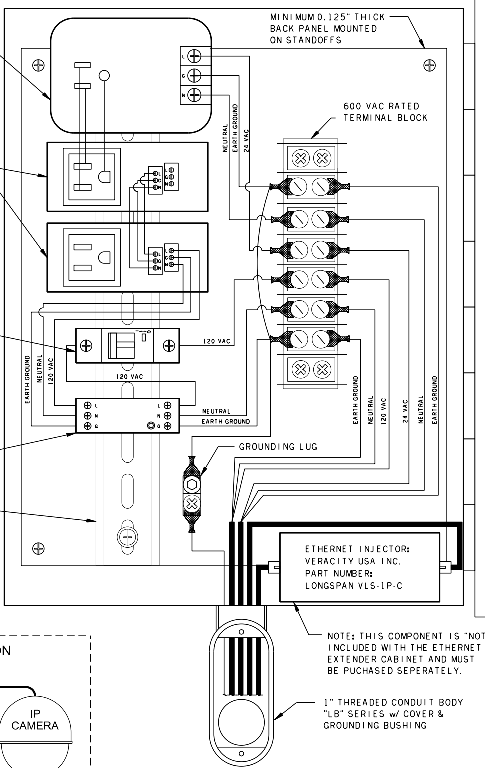
INTERIOR VIEW/WIRING DIAGRAM NTS
