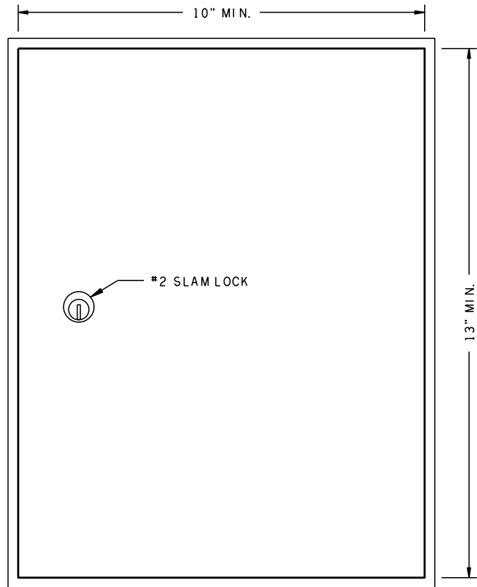
FRONT VIEW NTS
