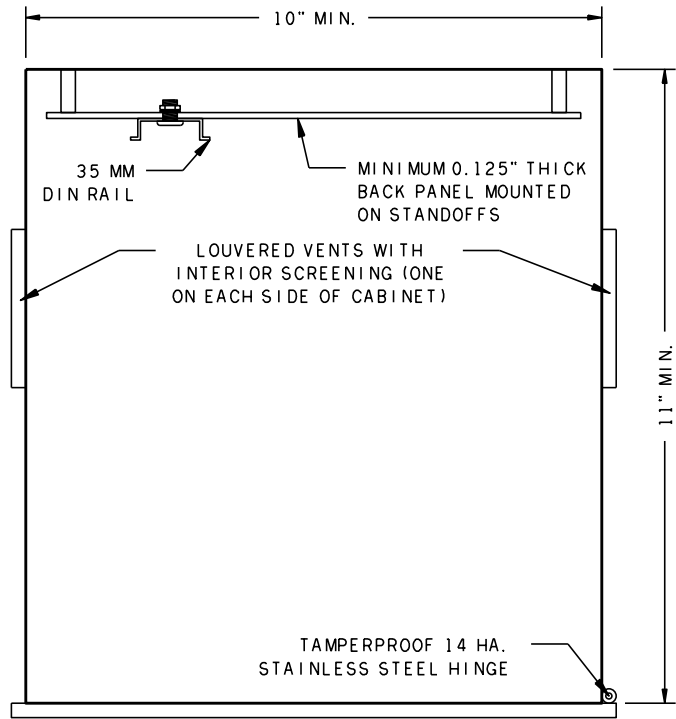
TOP VIEW NTS
